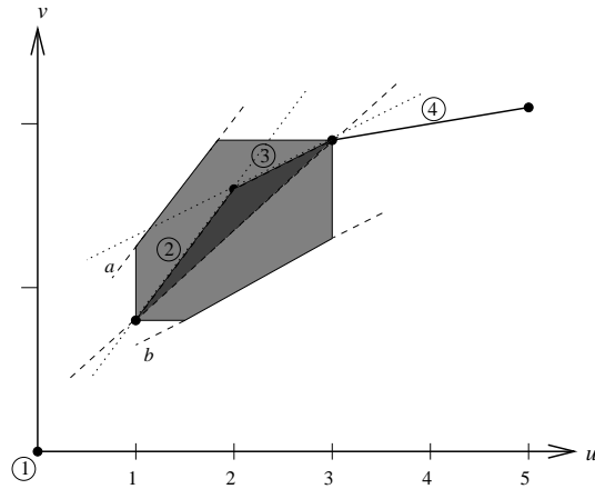
Figure 1. A piecewise linear function. The light grey area depicts the linear relaxation using variable subscripts, the dark grey area the relaxation obtained with the piecewise constraint.
