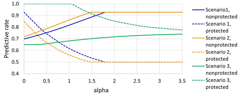
Fig. 9. Alpha fair predictive rates, assuming overall selection rate of 0.8.
