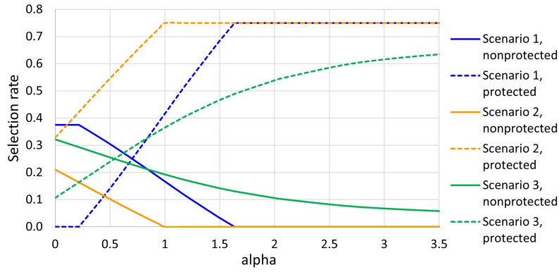
Fig. 2. Alpha fair selection rates, assuming overall selection rate of 0.25
